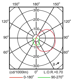
IFPS_TMS022 1xTL-D58W +GMS022 R-A-Polar Normal (separate)
