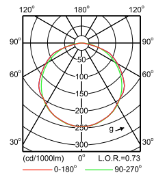
IFPS_TMS022 2xTL-D18W HFS +GMS022 R- Polar Normal (separate)
