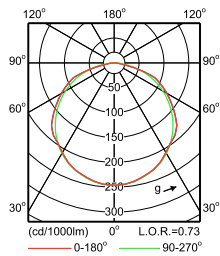
IFPS_TMS022 2xTL-D18W +GMS022 R-Polar Normal (separate)
