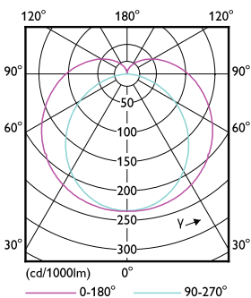
LEDtube MAS HF 14W G13 1000lm-LDD-LDD
