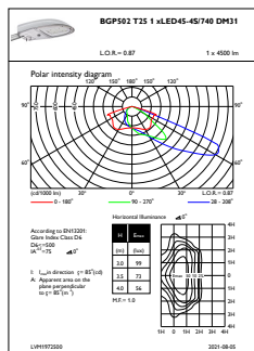
OFPL1_BGP502T251xLED45-4S740DM31
