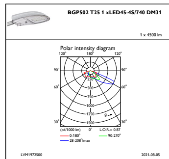
IFPC1_BGP502T251xLED45-4S740DM31
